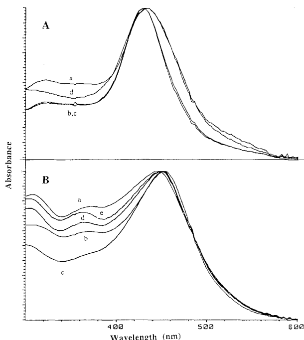
Fig. 2. Optical spectra of chromopeptides derived from trypsin digestion of cytochrome P460. Upper traces (A) are spectra recorded at t_R =19.22 (a), 19.59 (b), 19.84 (c), and 20.34 (d) min during the run on the gel filtration column. Lower traces (B) were recorded at t_R =13.91 (a), 14.22 (b), 14.68 (c), 15.25 (d), and 15.93 (e) min during the run on the reverse phase column.
